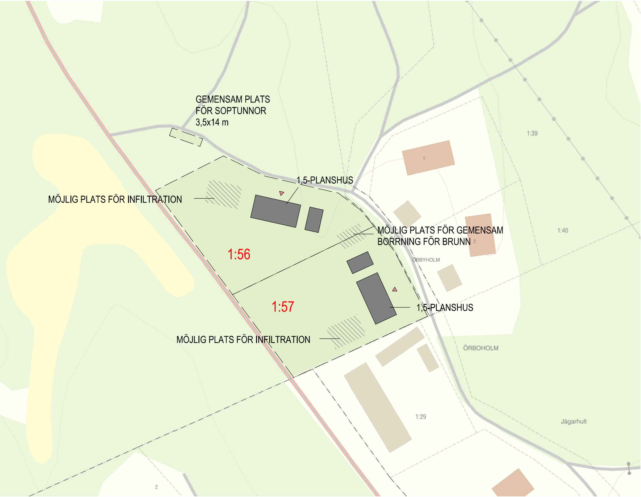
SITUATIONSPLAN 1:1000
